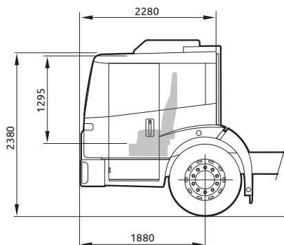
LOW CAB
