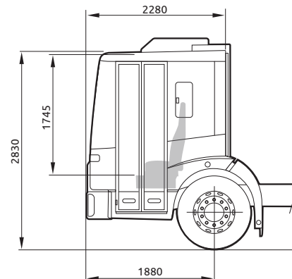
HIGH CAB
